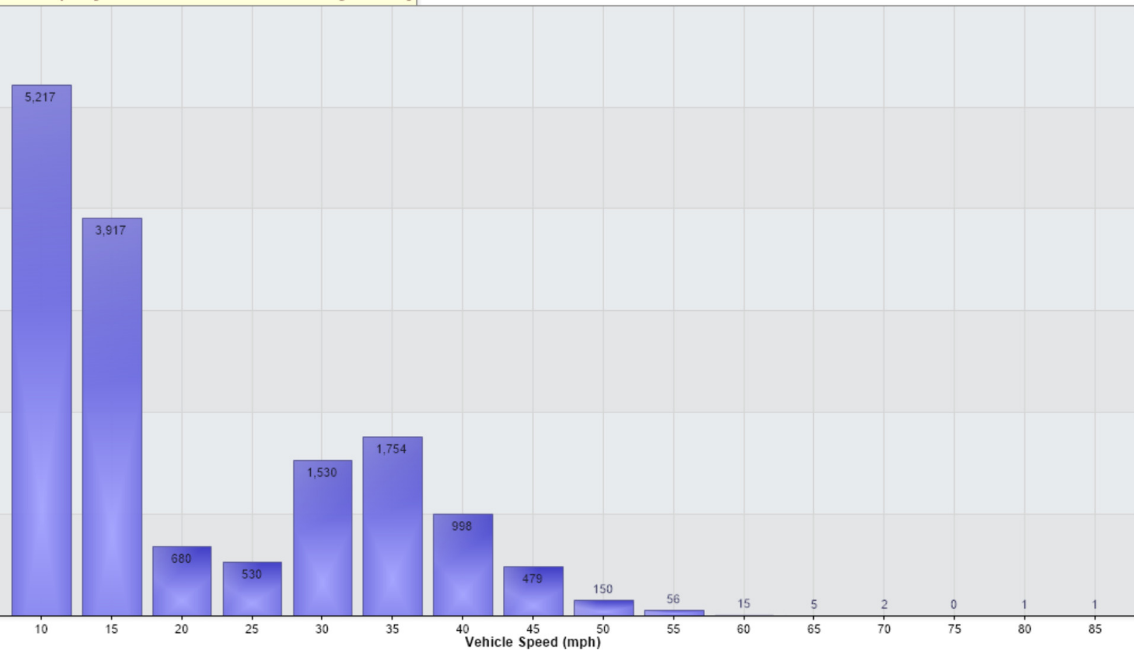
Vehicle Counts Vs. Speed [Mill Road Dec 2019-Jan 2020: Incoming Direction]
